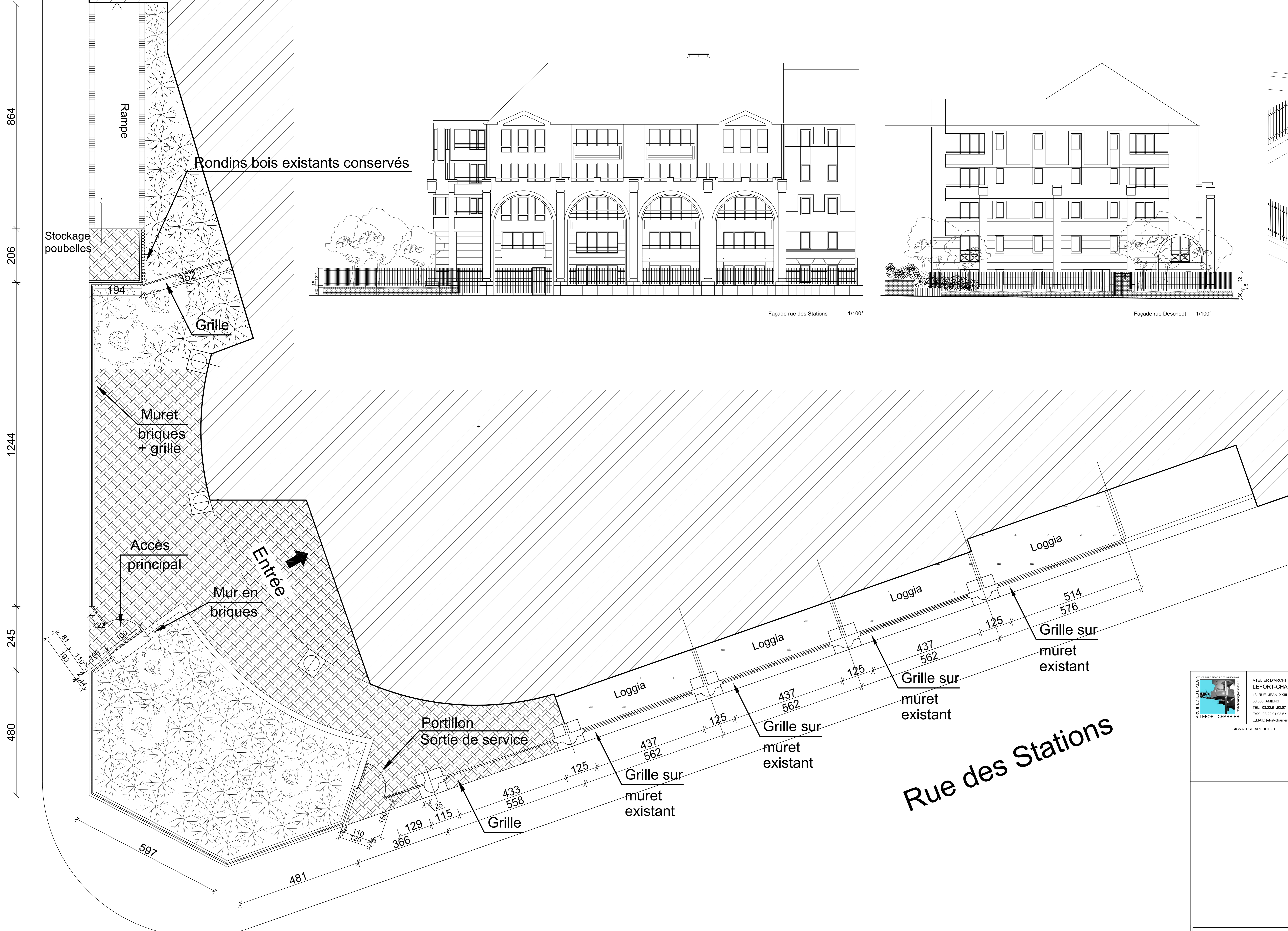
PLAN RDC / TERRASSES 1/50°
